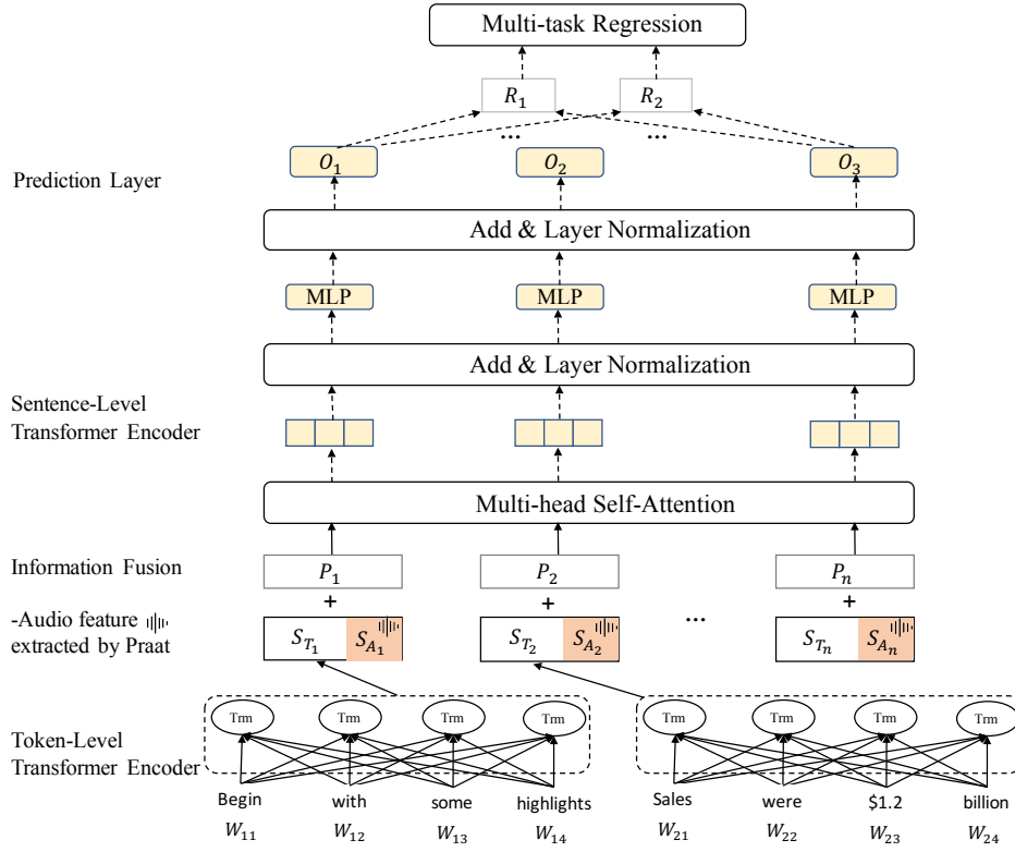
Figure 2: Hierarchical Transformer-based Multi-task Learning
