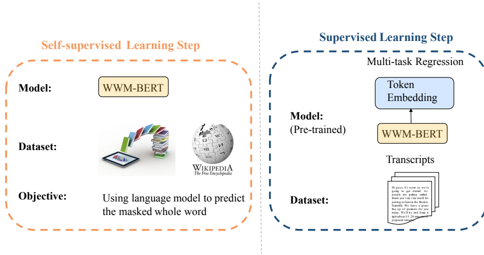
Figure 3: The pre-trained step in left is on-line available (trained on un-annotated data), and fine-tuning it on our prediction objectives.
