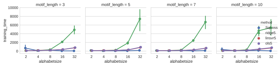
Fig. 2. Average training time (sec) across 5 runs, comparing the impact of varying data generation parameters (alphabet size, motif length) on 4 regression methods.
